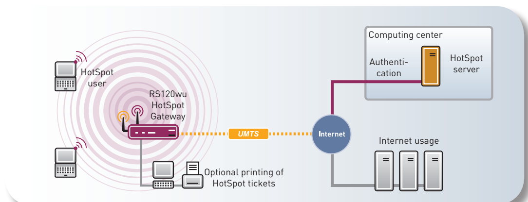
Mobile bintec HotSpot solution with an UMTS connection
